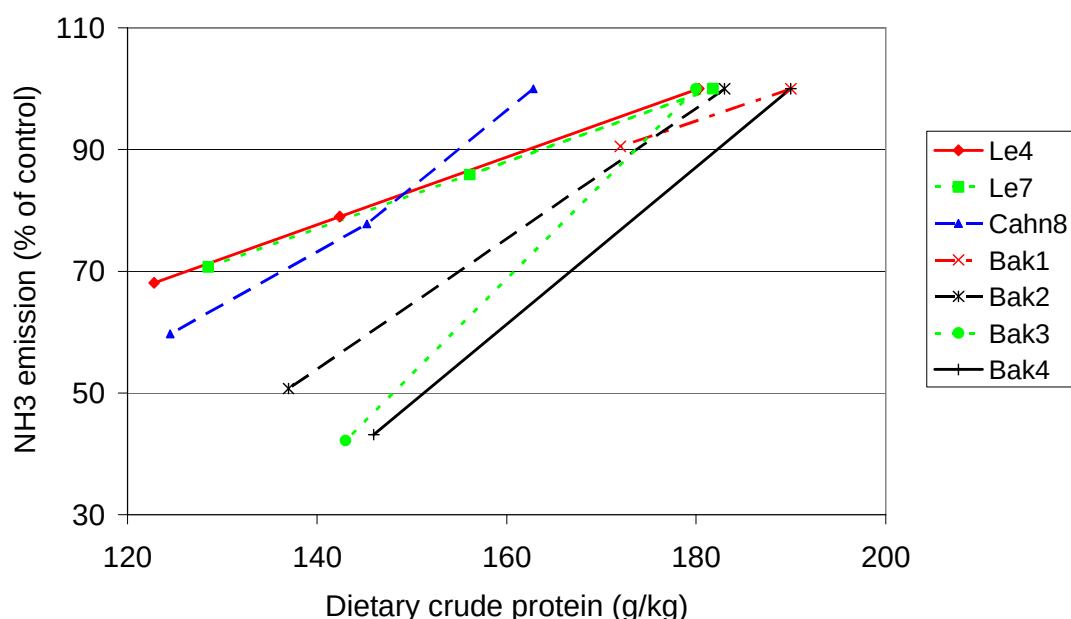
Figure 1. Relationship dietary protein level and NH 3 emission (Le, 2006; Canh, 1998; Bakker et al., 2004; number after name in legend indicates chapter or treatment).
